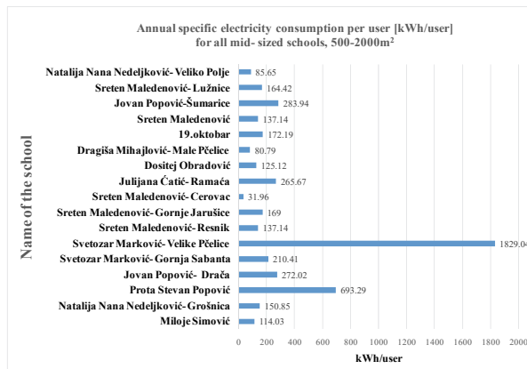
Fig. 6 – Annual specific electricity consumption per user [ \text{kWh/user} ] for all mid- sized schools, 500–2000 \text{m}^2 .
