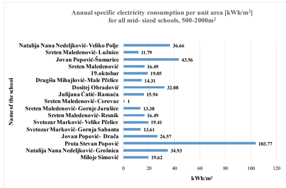
Fig. 5 – Annual specific electricity consumption per unit area [ \text{kWh/m}^2 ] for all mid- sized schools, 500–2000 \text{m}^2 .
