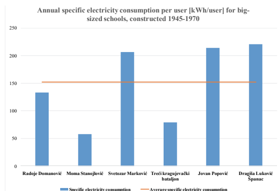
Fig. 18 – Annual specific electricity consumption per user [kWh/user] for big-sized schools, constructed 1945 – 1970.
