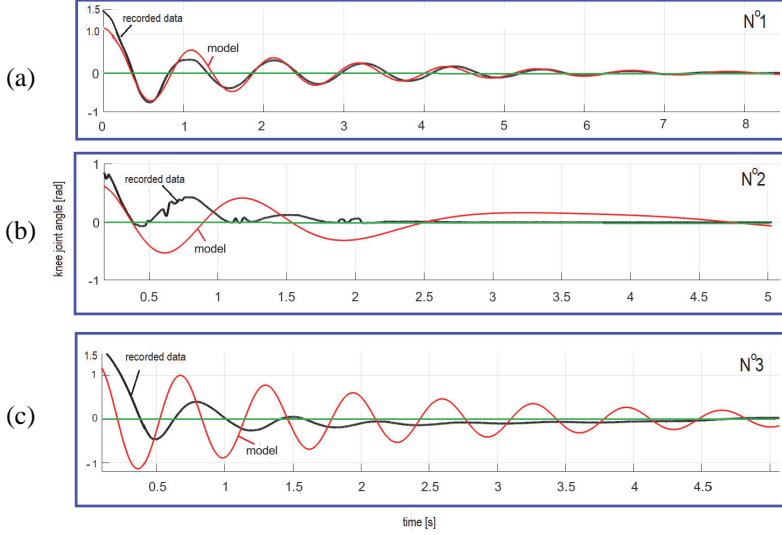
Fig. 8 – The estimated knee joint angles by using the linear model (red lines) superimposed over the recorded data for the patient with mild spasticity (Ashworth = 1) in the top panel, patient with extension spasticity (Ashworth = 4) in the middle panel, and patient with flexion spasticity (Ashworth = 4) in the bottom panel.
