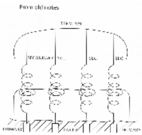
Fig. 22 – The complex excitation of Wardenclyffe transmitter for enabling both multichannel protection transmission and energy through generating complex waves (Source: Popovic Vojin, Nikola Tesla – From Colorado Springs to Long Island. Belgrade: The Nikola Tesla Museum, 2008, p.487).
