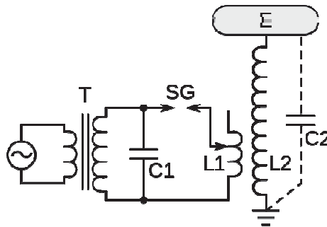
Fig. 2 – Basic electric shema of Tesla transformer.
