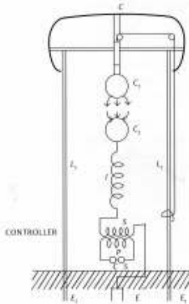
Fig. 26 – Tesla's drawing from notes, 29 th May 1901 in connection with new transmitter version in Wardenclyffe. He added the spark gap C_1 - C_2 and the spark gap ball distance adjustment wire. The internal independent supply represents the high-frequency transformer with special coil (Source: Popovic Vojin, Nikola Tesla – From Colorado Springs to Long Island. Belgrade: The Nikola Tesla Museum, 2008, p.496).
