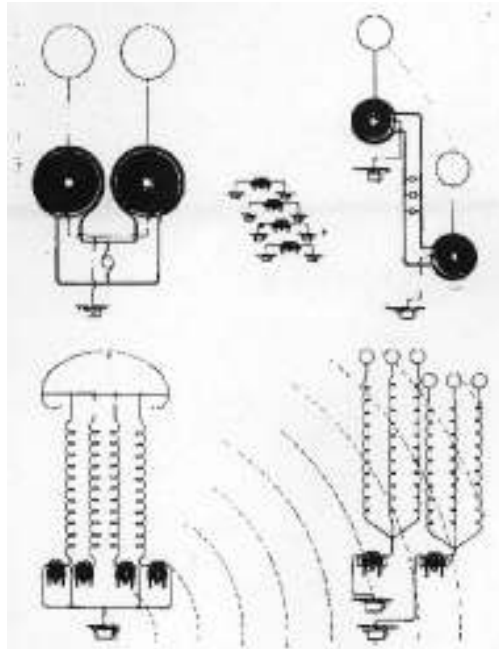
Fig. 23 – The outline of the signal transmitter and receiver from Tesla's uncompleted patent submission (most probably due to the unfinished transmitter in Wardencllyffe). The upper pictures: two coupled circuits transmitting the complex signal by means of "Hertzian" waves connected to the earth's ground. This outline was probably drawn for the sake of comparison with a new means of signal transmission in the pictures below. They were also put in order with the selective receiver. Lower pictures: the transmitter with four special coils (Wardencllyffe Tower) and receivers with three coils each for selective "current through ground" (Source: with the courtesy of The Nikola Tesla Museum in Belgrade).
