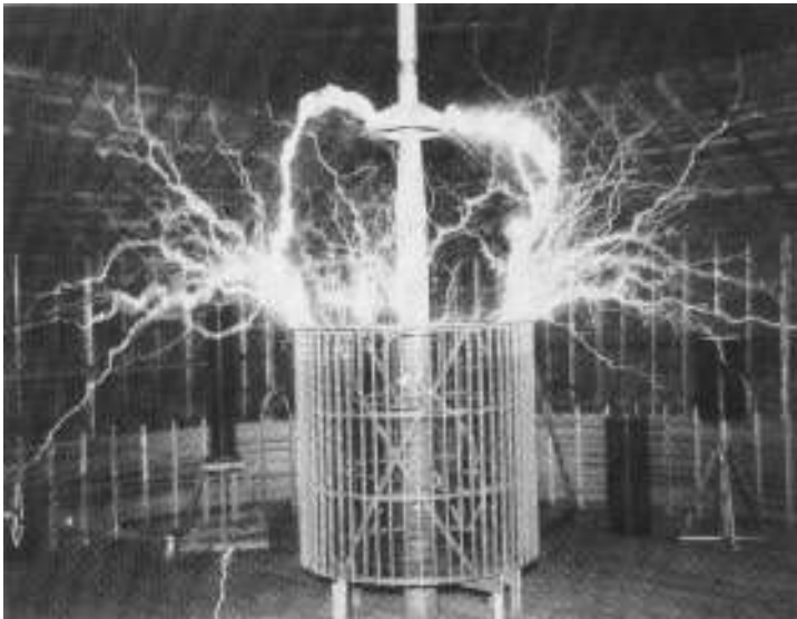
Fig. 14 – The special coil during the Colorado Springs experiment in 1899. Discharge between the coil top and the basis of an antenna metal part is visible. (Popovic Vojin, Nikola Tesla – From Colorado Springs to Long Island. Belgrade: The Nikola Tesla Museum, 2008, p.354).
