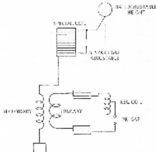
Fig. 10 – Basic electrical circuit diagram in the experiment on 5 October 1899 in a laboratory in Colorado Springs, which was used for the determination of the conditions for the formation of standing waves in a special coil (Source: Popovic, Vojin, Nikola Tesla - From Colorado Springs to Long Island , Belgrade, Nikola Tesla Museum, 2008, p.203).
