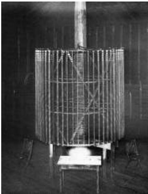
Fig. 13 – Special (extra) coil representing waveguide that is closed from the upper side by capacitance (the so-called shortened waveguide), while it is powered from the secondary of high-frequency transformer in its basis. The wire length is about 10% smaller than the quarter of the wavelength. (Source: Popovic Vojin, Nikola Tesla – From Colorado Springs to Long Island. Belgrade: The Nikola Tesla Museum, 2008, 340, p.336 and p.439).
