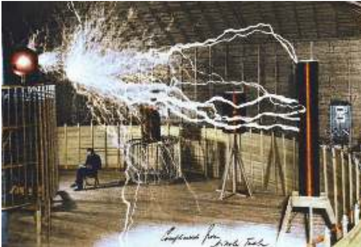
Fig. 15 – Electric discharge of approximately 7 m length with special coil in the laboratory center in Colorado Springs in 1899. The picture was made by means of double exposition so as to depict Tesla as being in the rear of discharge. Both special and right-hand narrow coils are in resonance.
