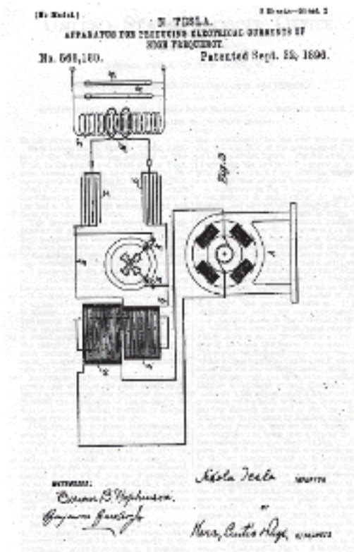
Fig. 1 – One of Tesla's patents of HF oscillator from 1896.
