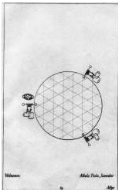
Fig. 25 – Tesla's drawing from the unpublished patent submission. Standing wave formation on the Earth's surface by means of three transmitters for wireless energy transmission. The surfaces with maximum energy density are within triangles while minimal density is within the hexagons. Courtesy of the Nikola Tesla Museum in Belgrade.
