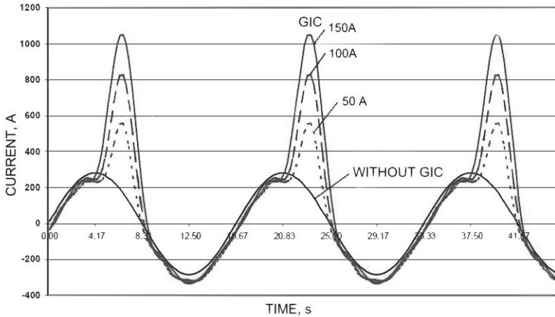
Fig. 4 – Steady-mode distortion of current shape in power transformer upon the flow of geomagnetic current of 50, 100 and 150A [4] within the transformer neutral conductor.
