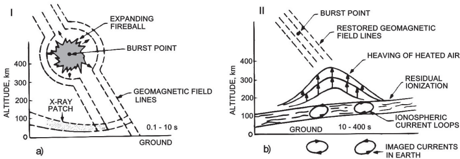
Fig. 1 – EMP MHD is consisted of two stages [2]: a) Blast Wave; b) Heave.
