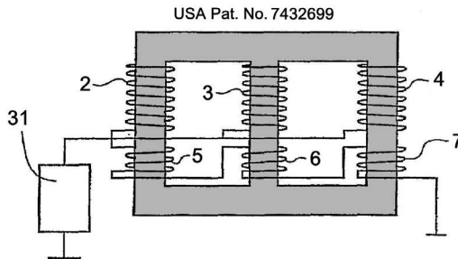
Fig. 8 – Power transformer with additional winding balancing GIC. 2-4 – basic winding; 5-7 – compensation winding; 31 – element with high DC resistance and low AC resistance.
