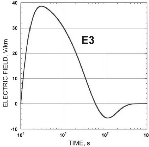
Fig. 2 – Changing horizontal component of electromagnetic field strength at the Earth's surface under the E3 component of nuclear detonation EMP [3].
