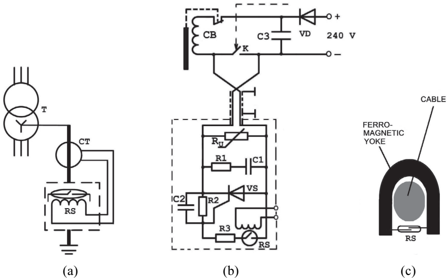
Fig. 10 – Power transformer protection relay protecting against low-frequency geomagnetic currents induced into the neutral circuit.
