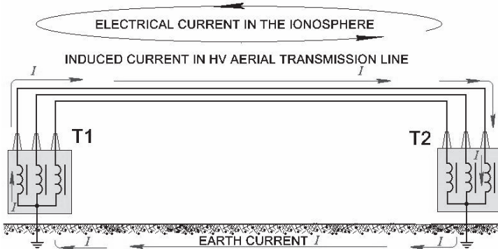
Fig. 3 – Flow chart of currents induced in electric mains and looped through the power transformer neutral conductor.
