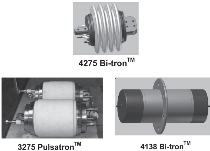
Fig. 6 – High-power high-voltage controlled arresters by Advanced Fusion Systems types 4275 (35 kV, 100 kA); 3275 (500 kV, 250 kA); 4138 (75 kV, 250 kA).
