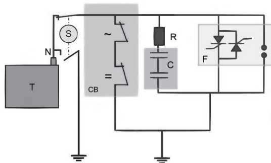
Fig. 5 – Typical design of the device blocking GIC in the neutral conductor of power transformer . T – transformer; S – switching apparatus designed for making the device inoperative; CB – special circuit breaker designed for disconnecting AC/DC; C – capacitors bank; R – current limiting resistor; F – special protection against overvoltage under emergency currents in neutral circuits.
