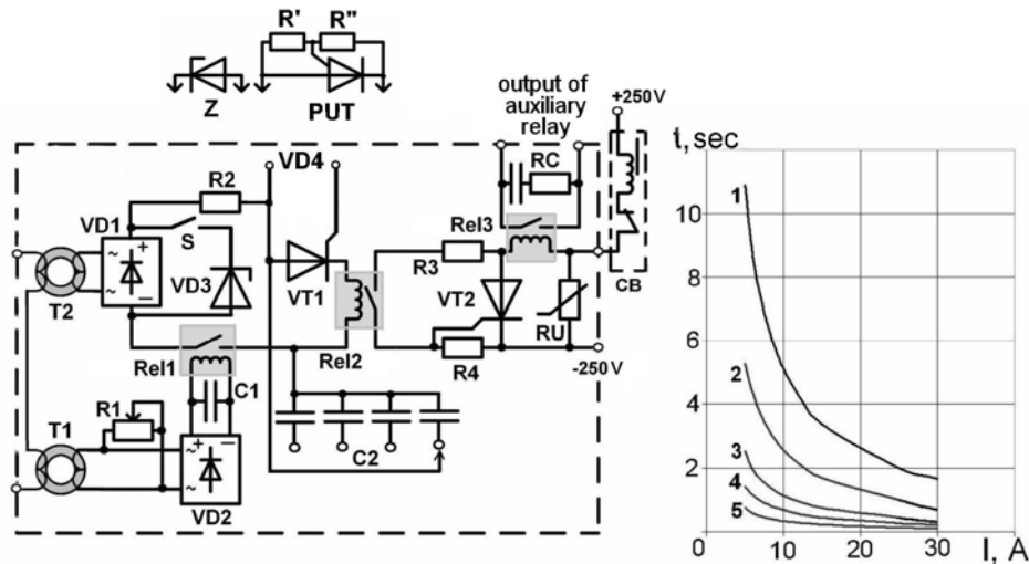
Fig. 6 – Universal protective current relay with the time delay: the basic circuit diagram and set of experimental time-current characteristic curves. For the relay with the dependent time-current characteristic curves the various values of capacity C_2 (in \mu F ) are as follows: 1 - 4400; 2 - 3200; 3 - 2200; 4 - 1000; 5 - 300.
