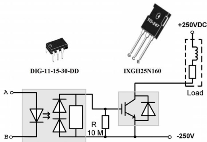
Fig. 5 – An embodiment of output switching unit of the relay based on the modern IGBT-transistor (IXGH25N160) and specialized driver with the dynamic discharging (DIG-11-15-30-DD) for this transistor control.
