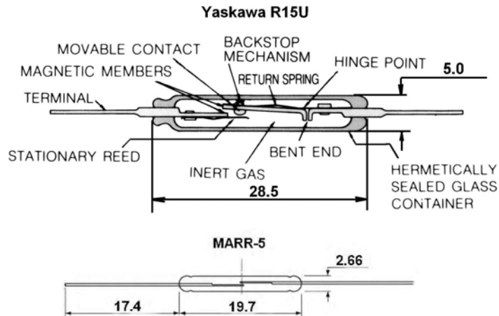
Fig. 1 – Modern reed switches, recommended for use in the protective relays. At the top: gas filled power reed switch R15U (Yaskawa); at the bottom: miniature high-speed vacuum reed switch MARR-5 (Hamlin Inc.).
