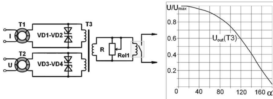
Fig. 7 – The relay of power direction: basic circuit diagram of measuring the threshold module and experimental dependence of an output voltage of transformer T3 on an angle shift between two voltages on its primary windings.
